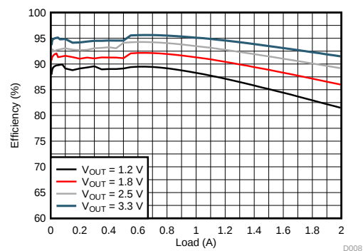
Efficiency at 5-V Input Voltage
