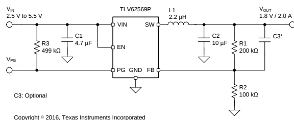
Simplified Schematic
