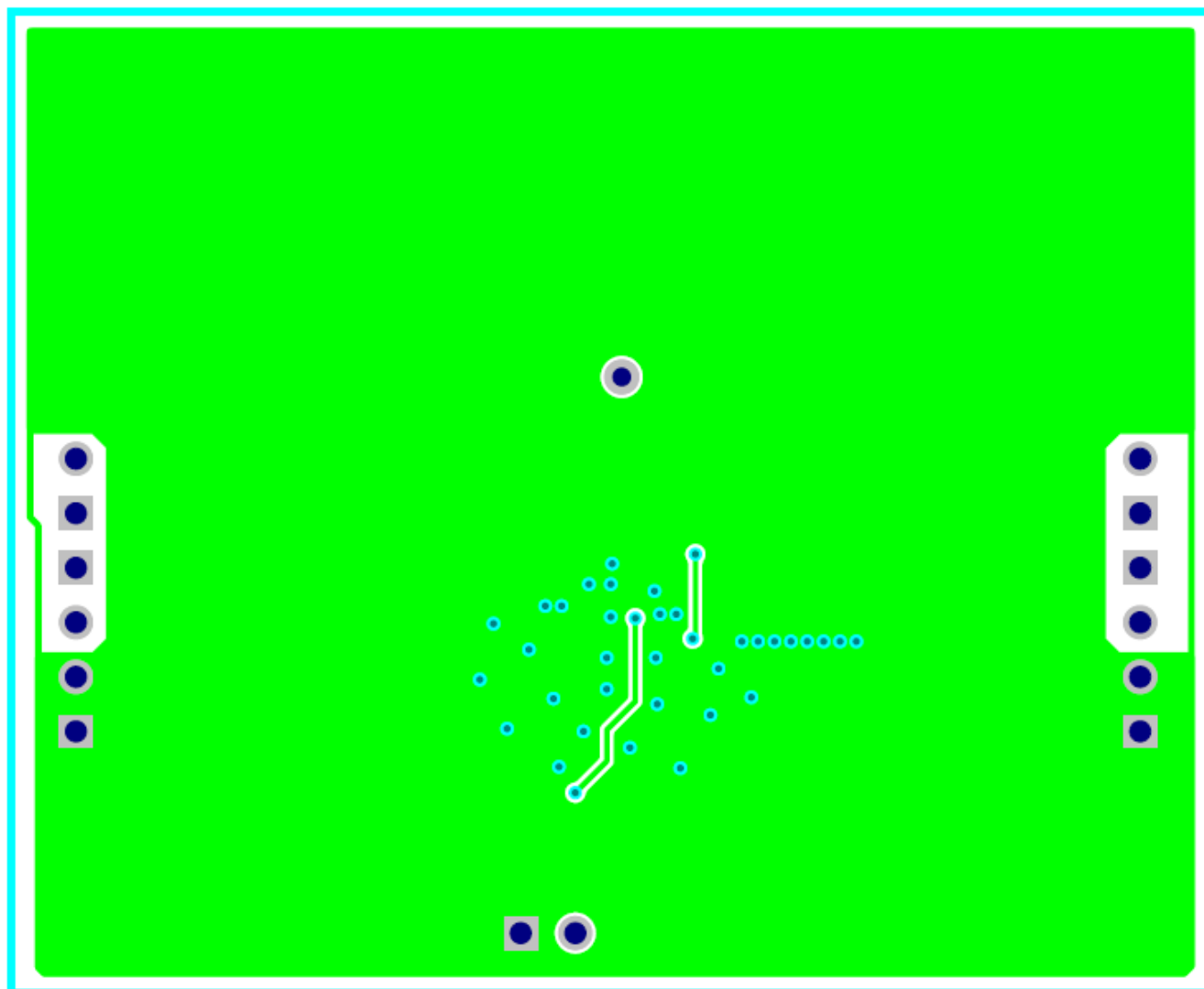
Figure 5. Bottom Layer
