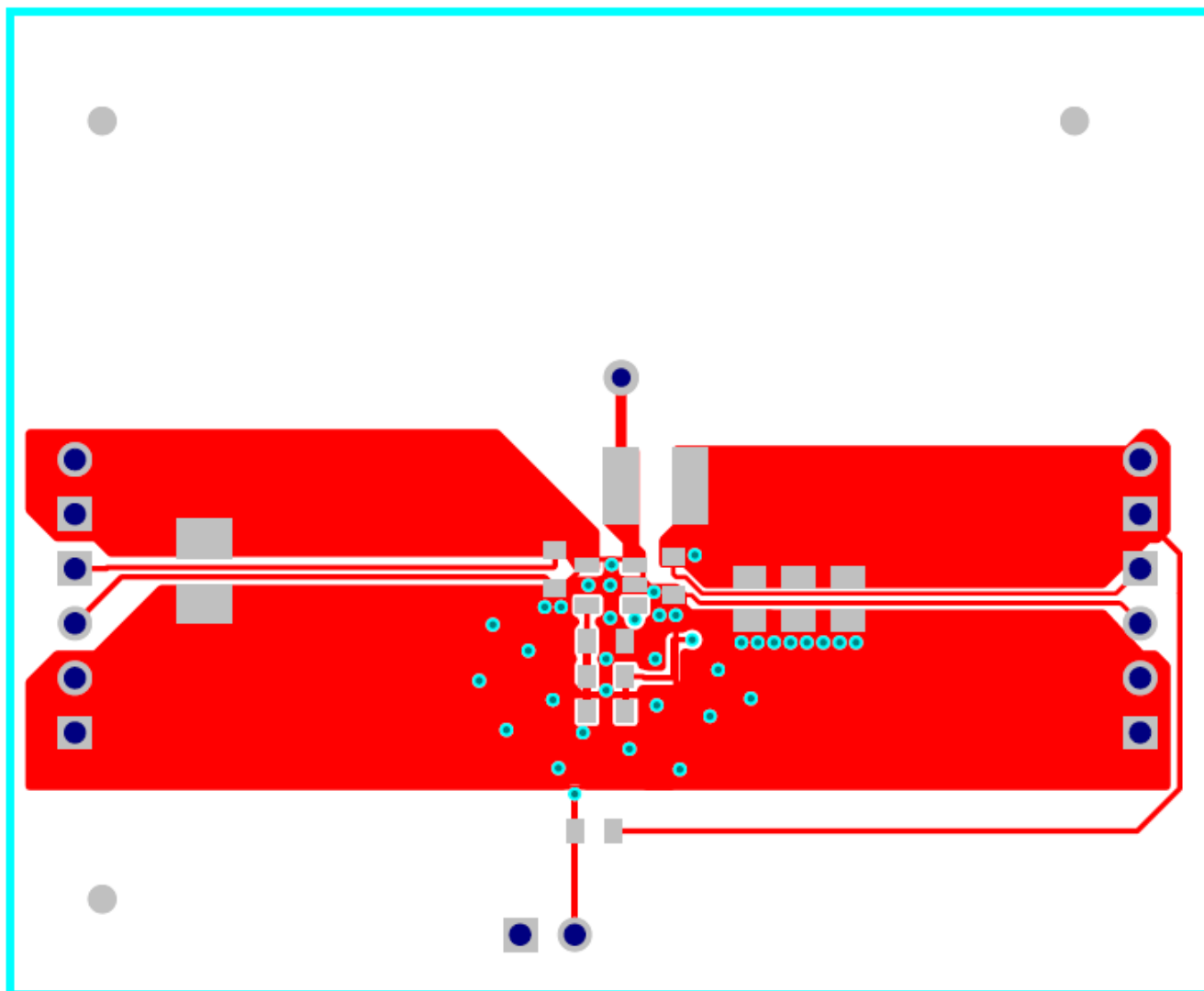
Figure 4. Top Layer
