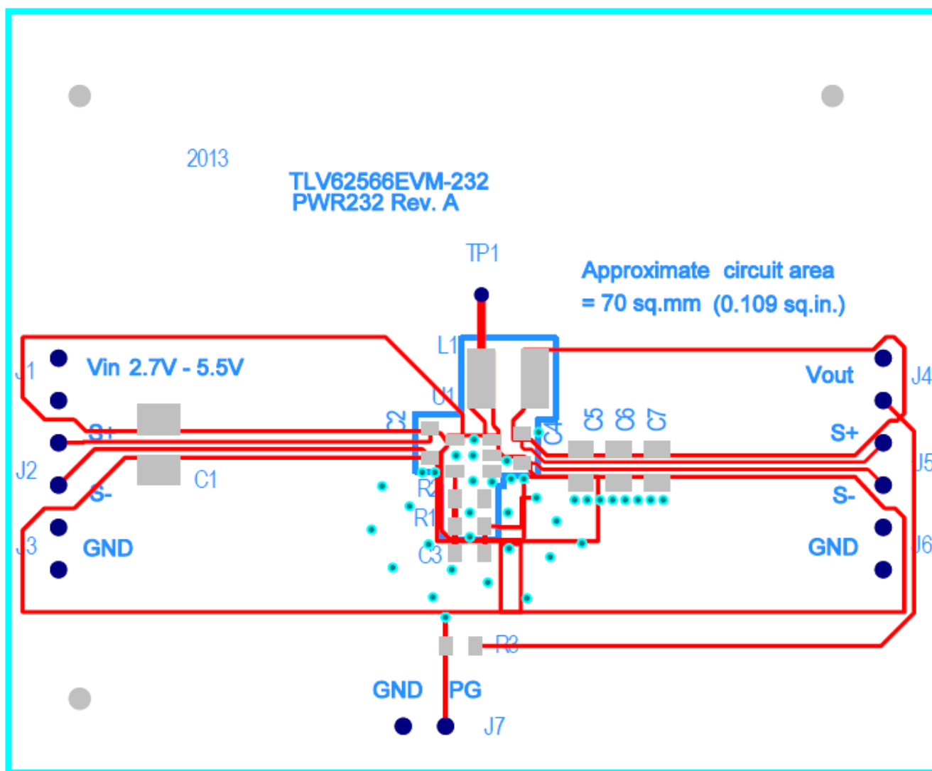
Figure 2. Assembly Layer
