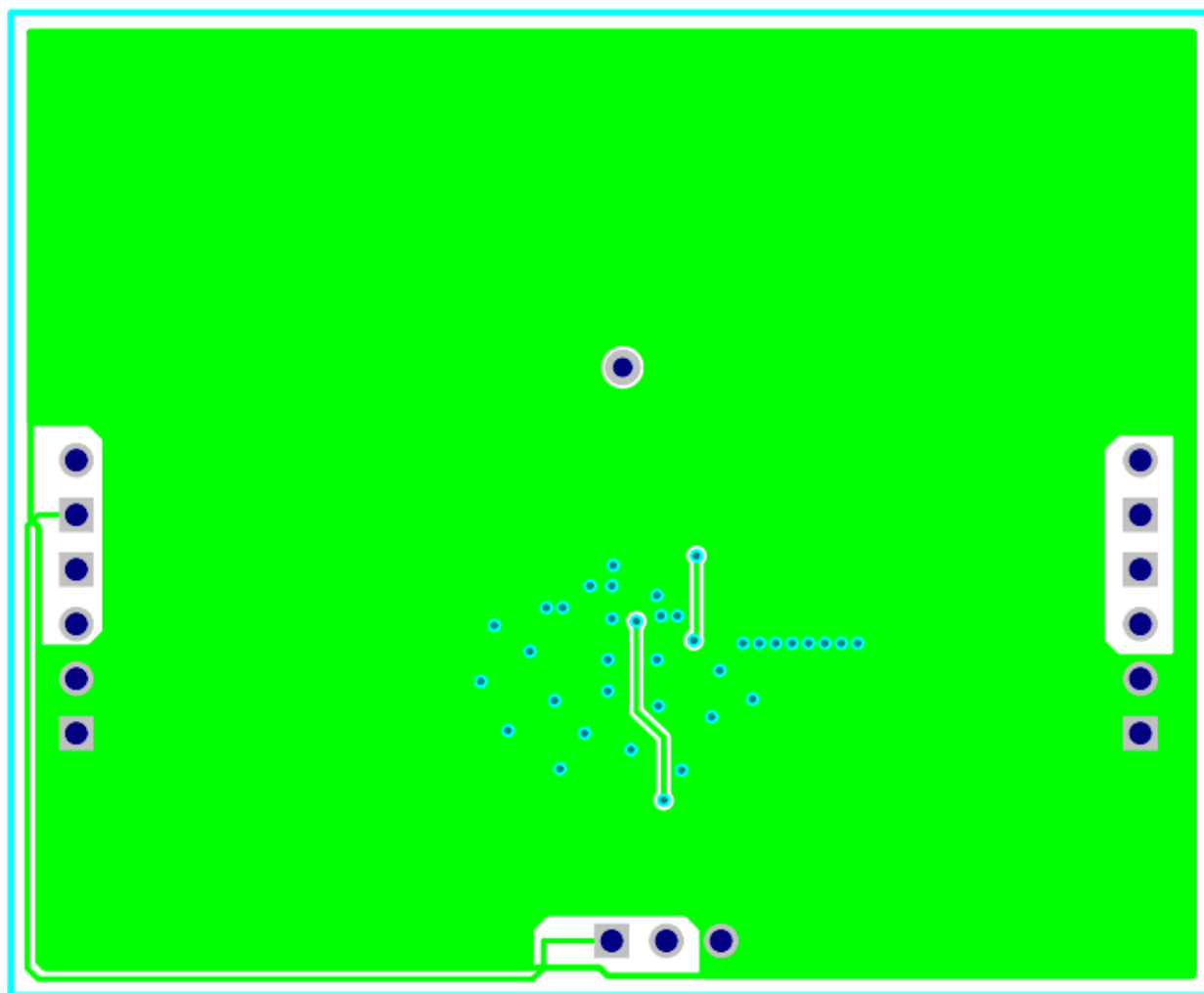
Figure 5. Bottom Layer
