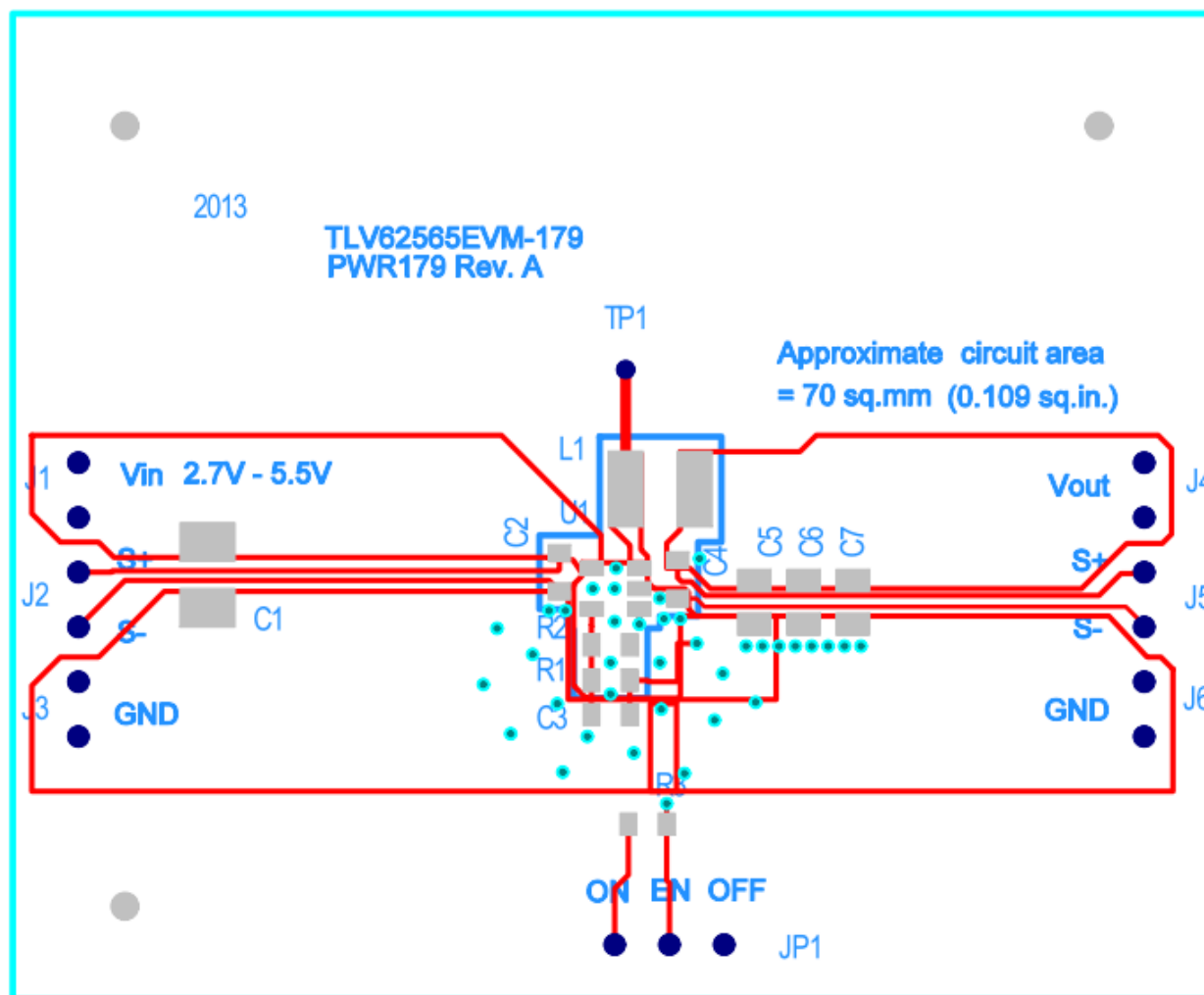
Figure 2. Assembly Layer
