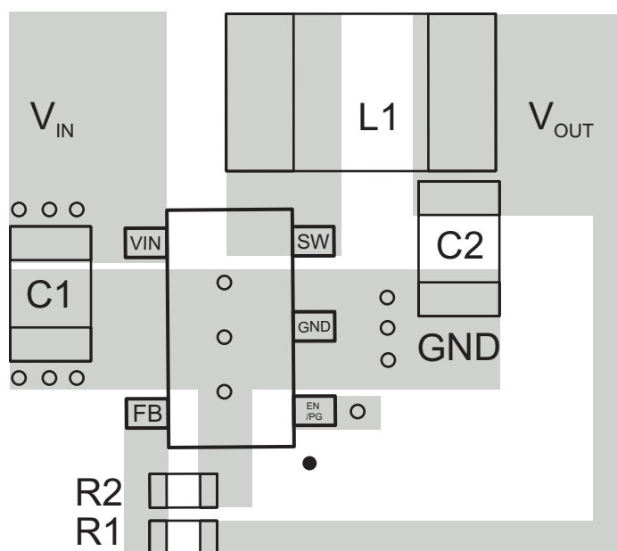
Figure 22. TLV62565/6 Layout
