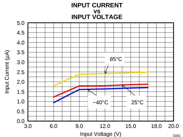
Figure 21. Shutdown Current
