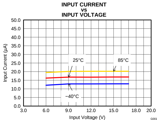
Figure 20. Quiescent Current
