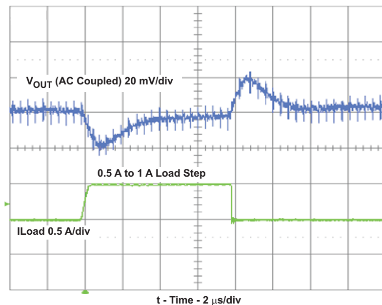
Figure 12. Load Transient Response With 2.2-μH Inductor and V IN = 12 V
