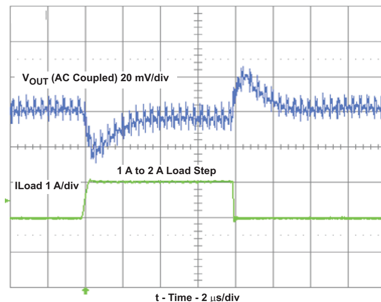
Figure 11. Load Transient Response With 1-μH Inductor and V IN = 12 V
