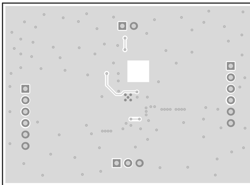
Figure 4. Bottom Layer
