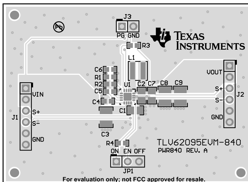
Figure 1. Top Assembly
