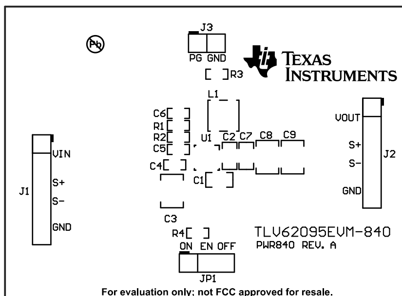
Figure 2. Top Overlay
