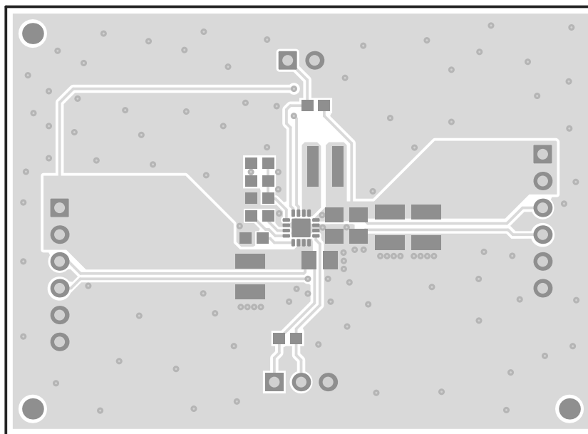
Figure 3. Top Layer
