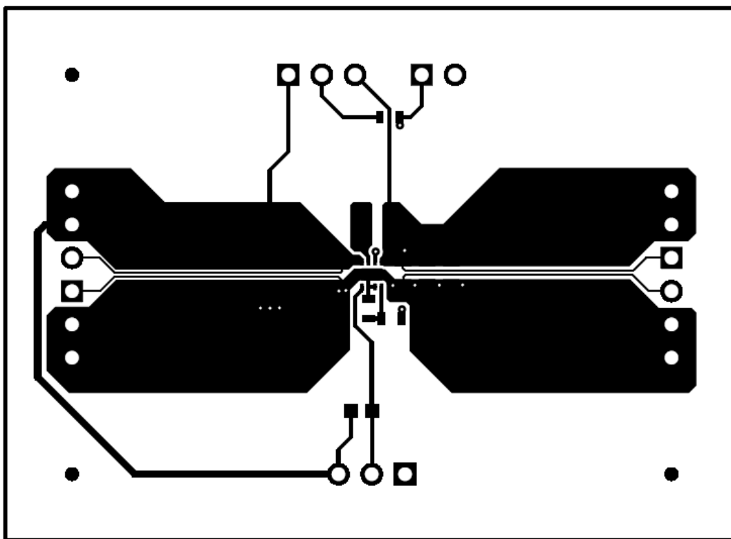
Figure 2. Top Layer
