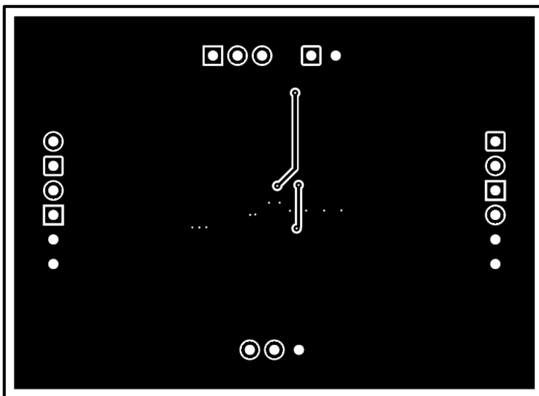
Figure 3. Bottom Layer
