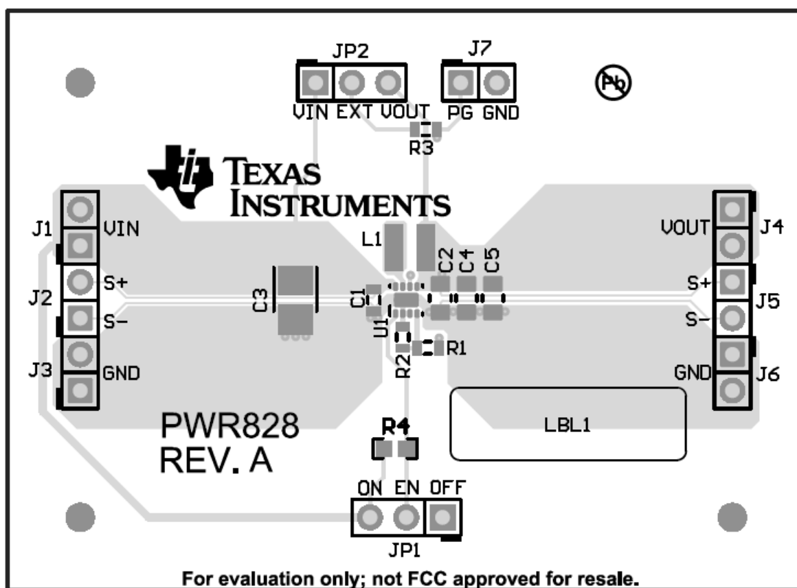
Figure 1. Assembly Layer
