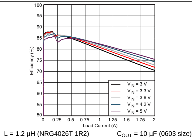
Figure 3. Efficiency vs Load Current Auto PFM and PWM MODE
