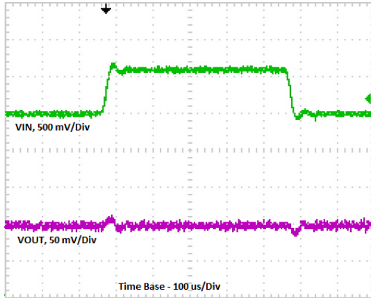
Figure 13. Line Transient Response PWM Mode
