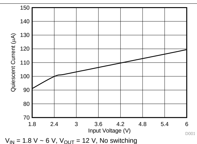
Figure 6. Quiescent Current into VIN vs Input Voltage
