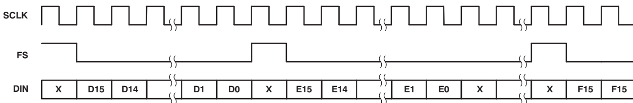
Figure 9. Timing Diagrams
