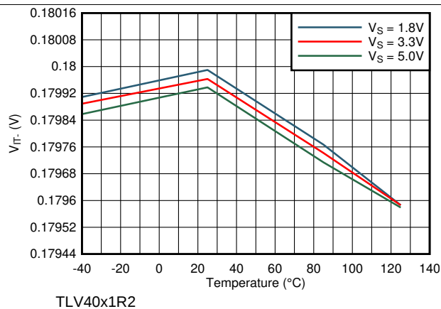
Figure 10. Negative Threshold vs Temperature
