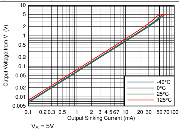
Figure 26. Output Voltage vs Output Sinking Current
