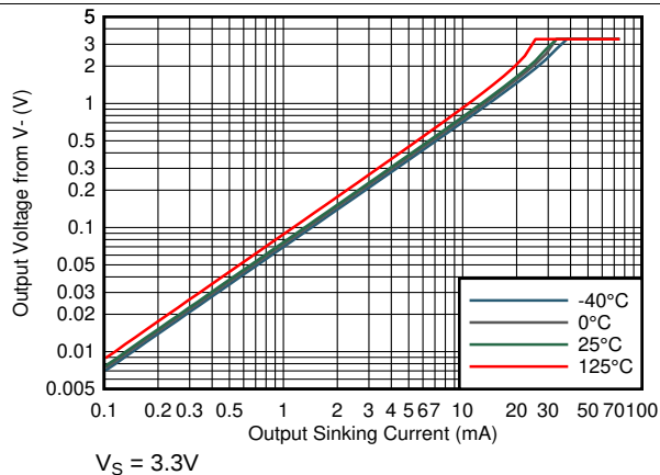
Figure 24. Output Voltage vs Output Sinking Current
