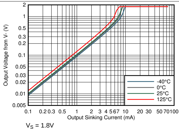
Figure 22. Output Voltage vs Output Sinking Current
