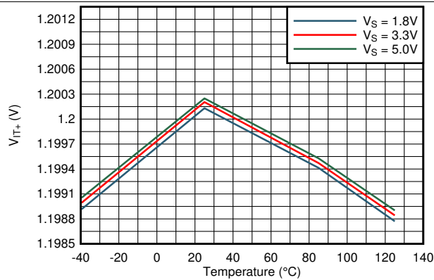
Figure 2. Positive Threshold vs Temperature
