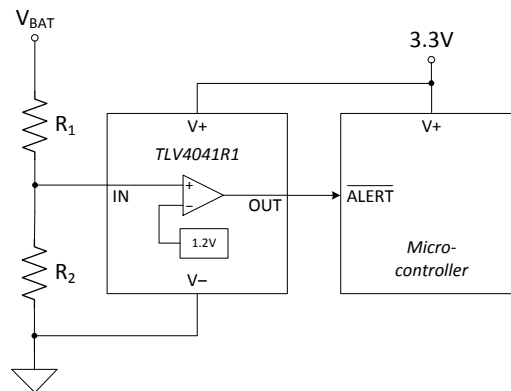
Figure 44. Under-Voltage Detection
