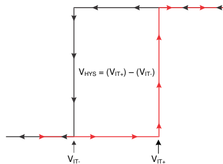
Figure 37. Transfer Curve
