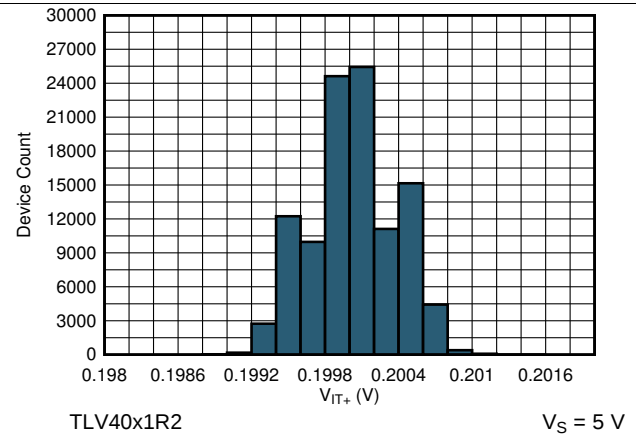
Figure 9. Positive Threshold Histogram
