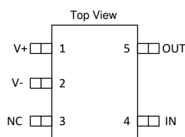
SOT-23 Pin Functions
