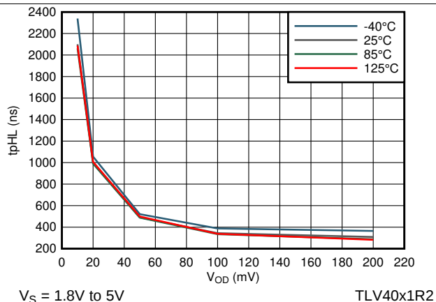
Figure 30. Propagation Delay High-Low vs Input Overdrive
