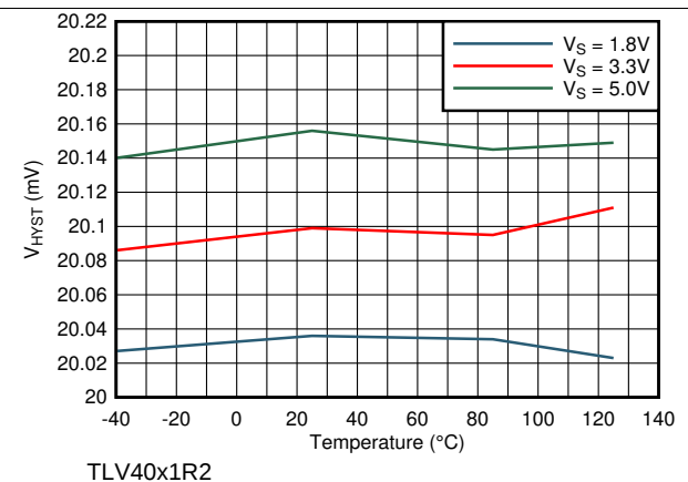
Figure 12. Hysteresis vs Temperature
