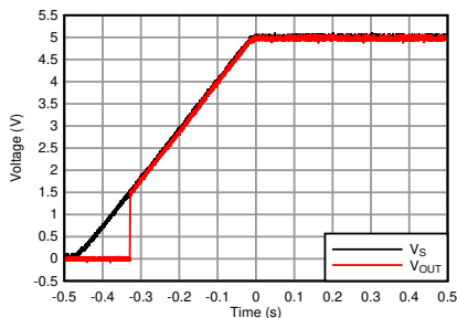
Figure 35. TLV4041/4051 Output for V_S Rising
