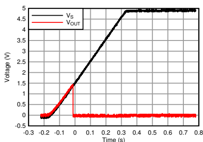
Figure 33. TLV4021/4031 Output for V_S Rising
