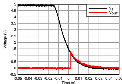
Figure 34. TLV4021/4031 Output for V_S Falling
