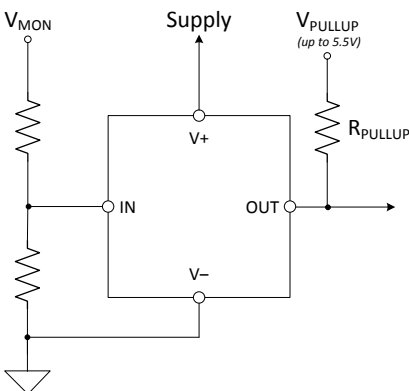
Figure 43. Level-Shifting
