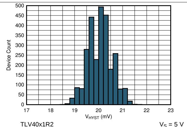
Figure 13. Hysteresis Histogram
