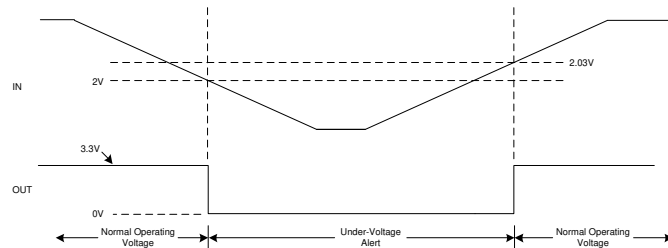
Figure 45. Under-Voltage Detection
