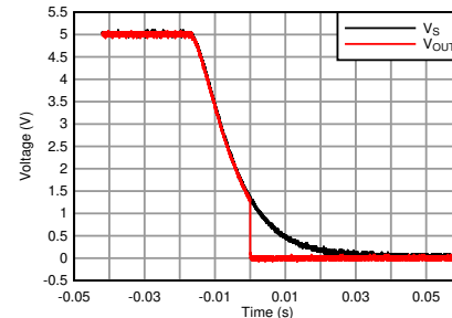
Figure 36. TLV4041/4051 Output for V_S Falling
