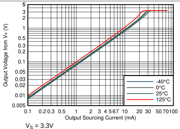
Figure 25. Output Voltage vs Output Sourcing Current
