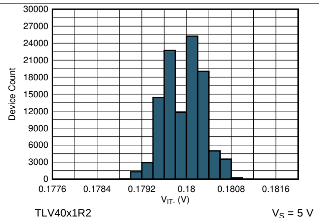
Figure 11. Negative Threshold Histogram
