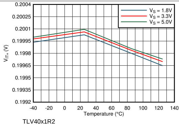
Figure 8. Positive Threshold vs Temperature
