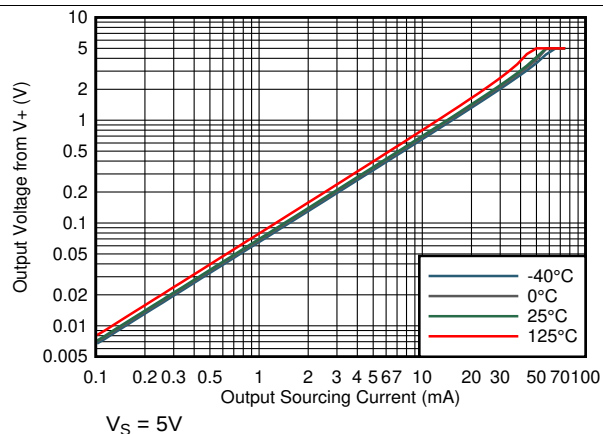
Figure 27. Output Voltage vs Output Sourcing Current
