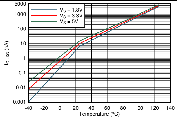
Figure 21. Output Current Leakage vs Temperature
