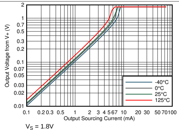
Figure 23. Output Voltage vs Output Sourcing Current
