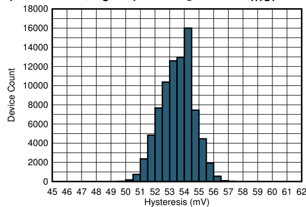
Figure 40. V_{HYST} Histogram (TLV40x1S5, V_S=5V )
