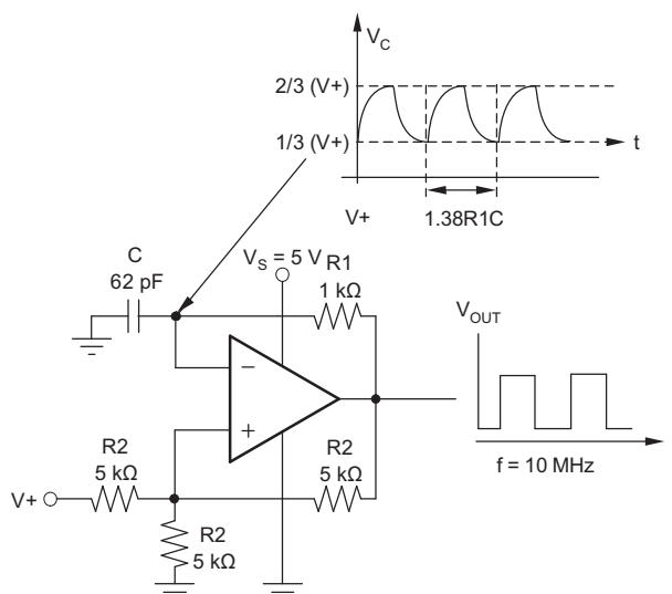
Figure 16. Relaxation Oscillator
