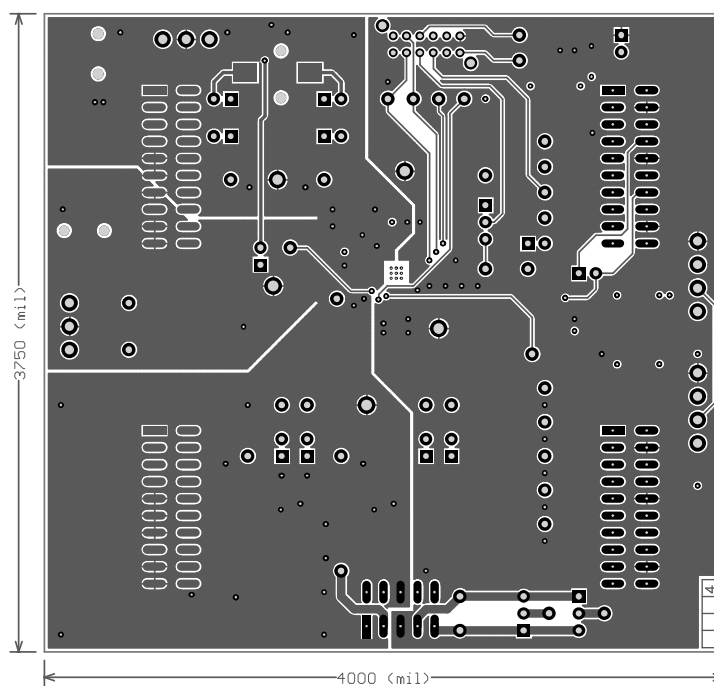
Figure 15. Bottom Layer
