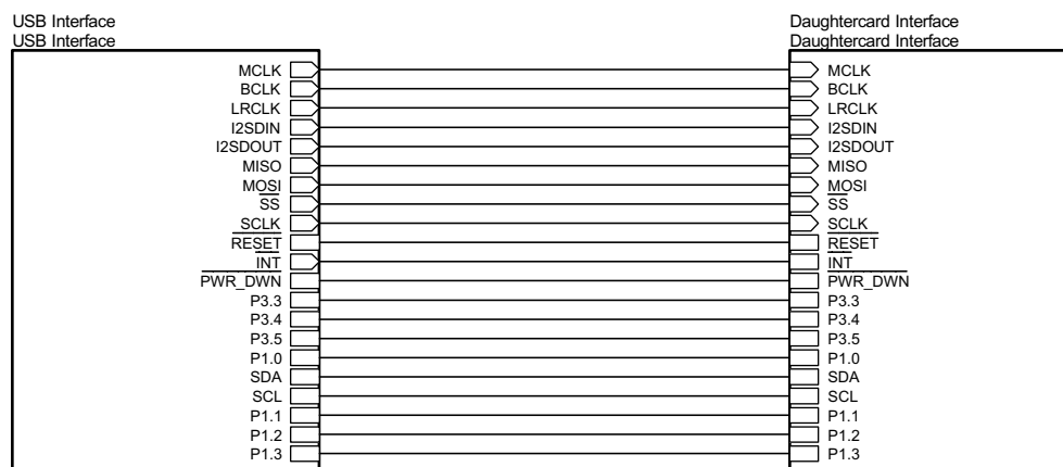
Figure 20. USB-MODEVM Schematic (Sheet 1 of 3)
