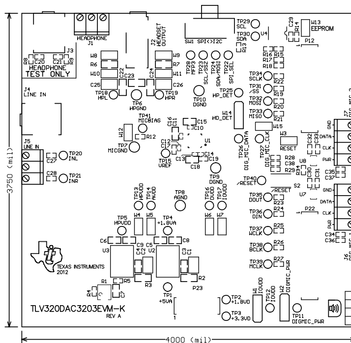
Figure 16. Top Overlay
