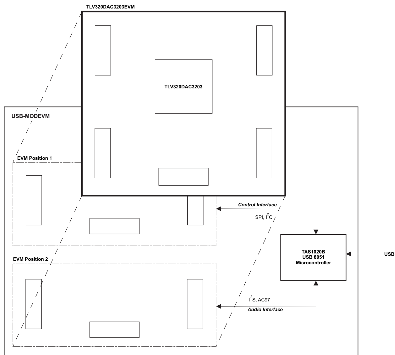
Figure 1. TLV320DAC3203EVM-K Block Diagram
