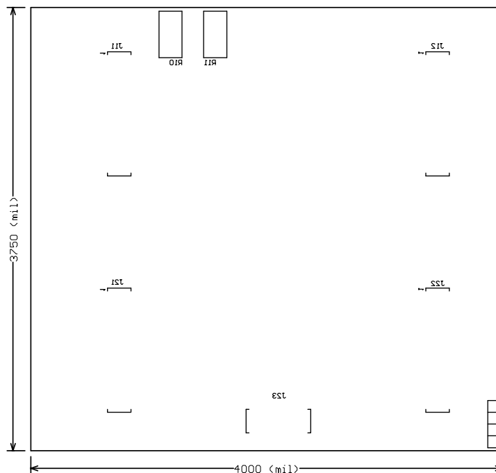
Figure 17. Bottom Overlay
