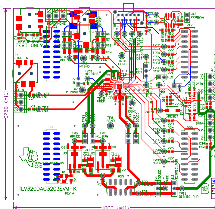
Figure 19. Composite
