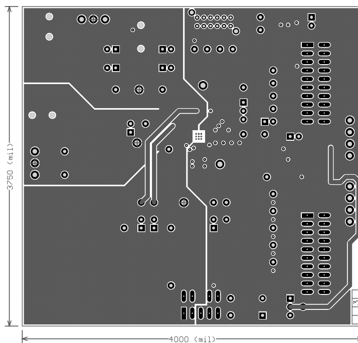
Figure 14. Mid-Layer 2
