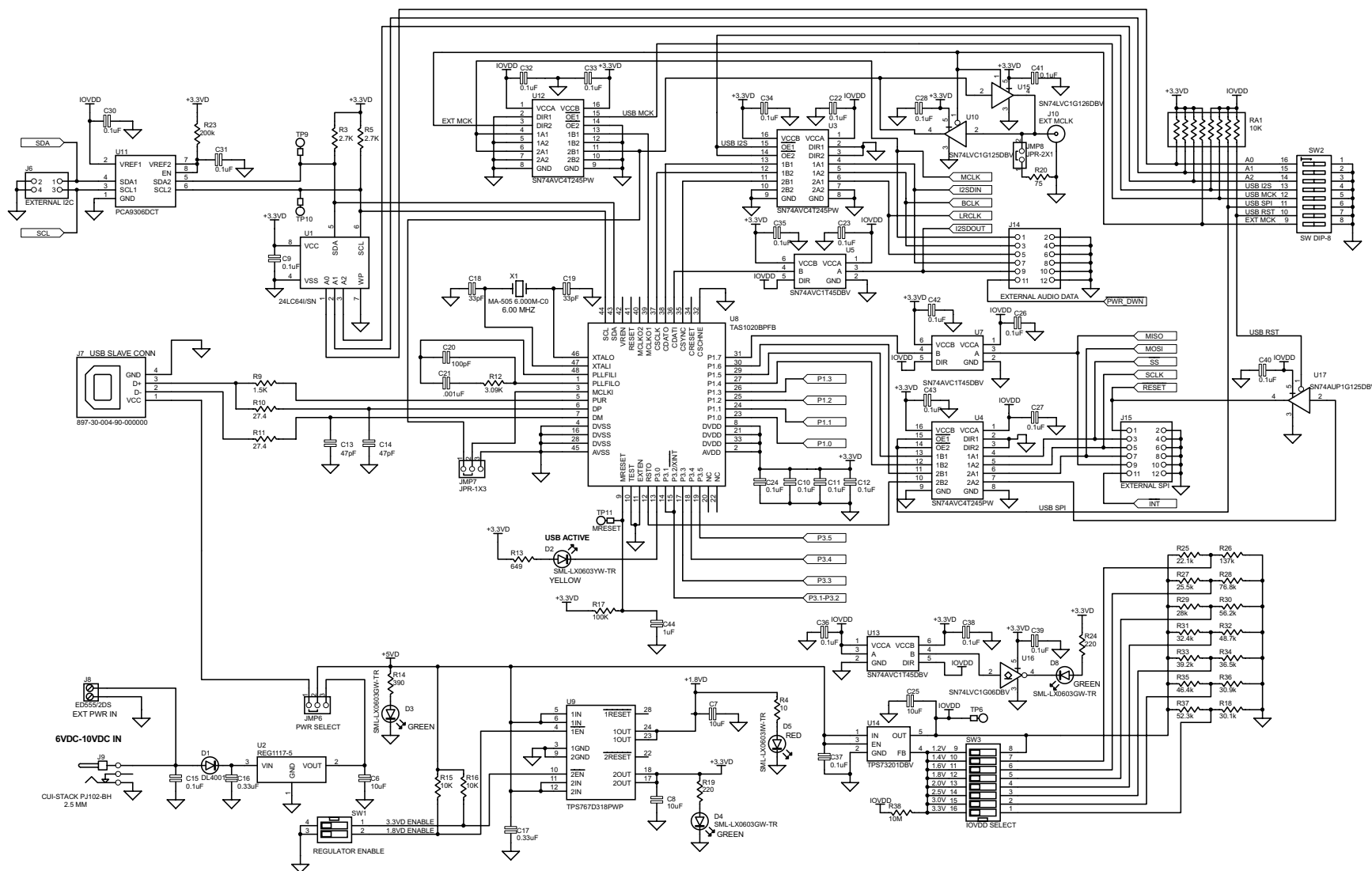
Figure 21. USB-MODEVM Schematic (Sheet 2 of 3)
