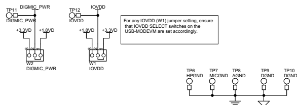
Figure 11. TLV320AIC3253EVM Schematic (Sheet 2 of 2)
