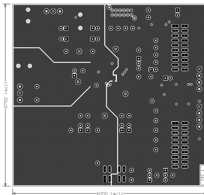
Figure 13. Mid-Layer 1
