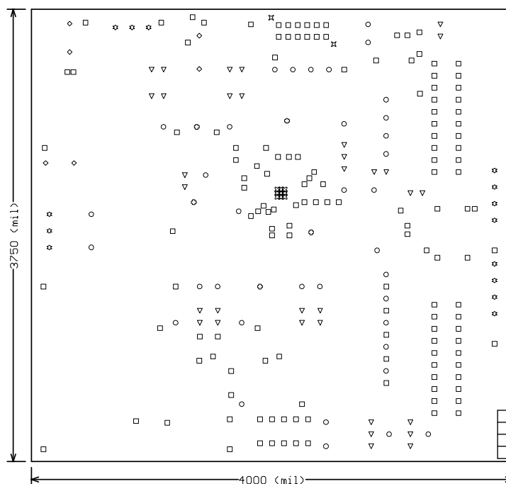
Figure 18. Drill Drawing
