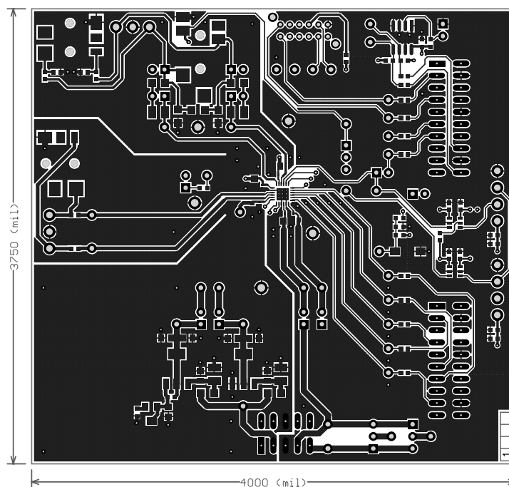
Figure 12. Top Layer
