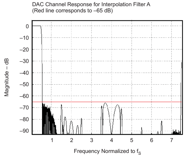
Figure 55. DAC Interpolation Filter A, Frequency Response
