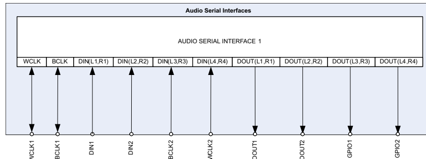
Figure 85. Multi-channel, Multi-Terminal Inputs and Outputs to Audio Serial Interface 1
