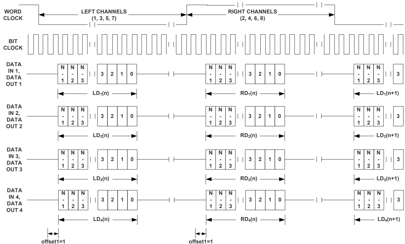
Figure 107. I²S Timing for Multi-channel Mode, Four Data Lines with Offset1=1
