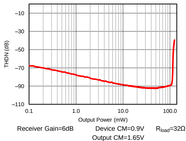
Figure 31. DAC Playback on Receiver Amplifier, Total Harmonic Distortion + Noise versus Output Power
