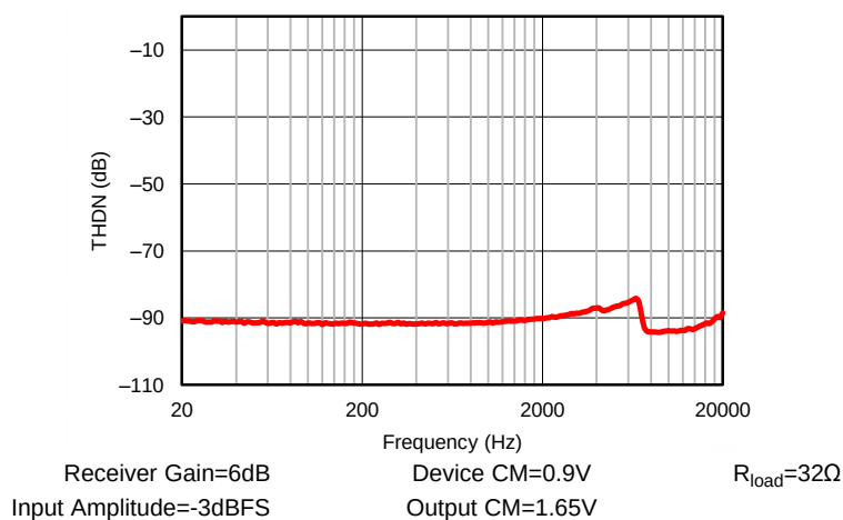
Figure 32. DAC Playback on Receiver Amplifier, Total Harmonic Distortion + Noise versus Input Frequency
