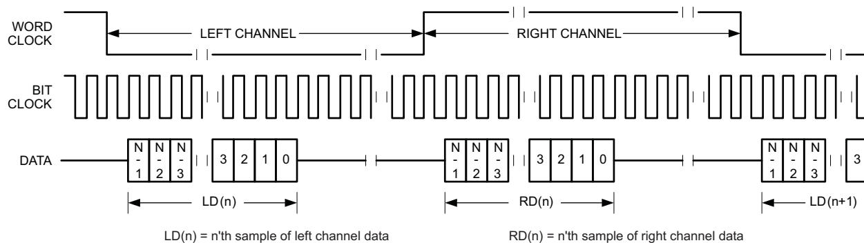
Figure 7-45. Timing Diagram for I 2 S Mode With Offset = 0 and Bit Clock Inverted
