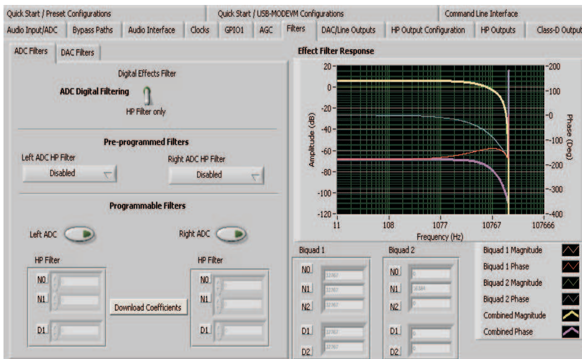
Figure 14. Filters Tab
