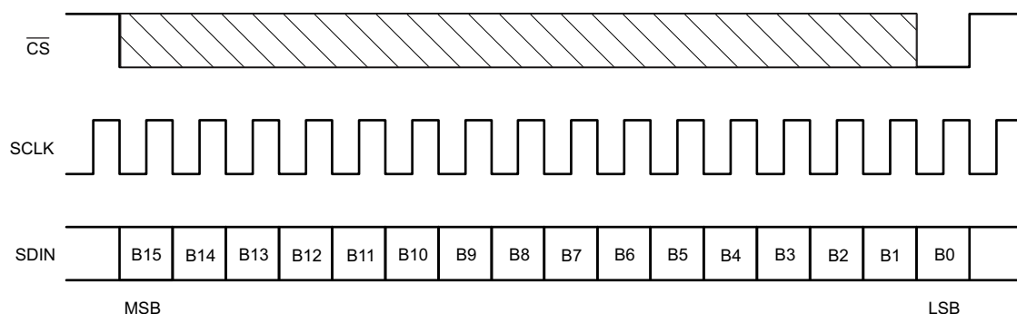
Figure 3-1. SPI Timing
