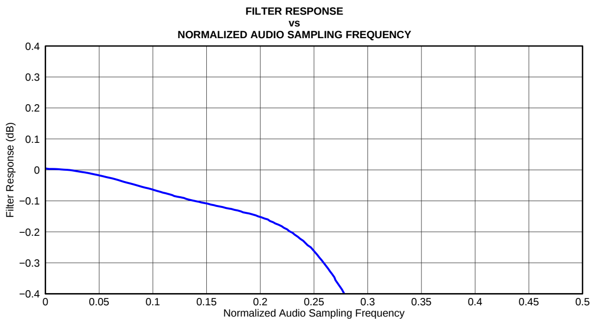
Figure 3-26. DAC Digital Filter Ripple 3: USB Mode Only
