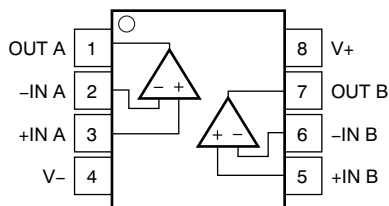
TLV2316-Q1 DGG Package 8-Pin VSSOP Top View
