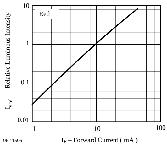
Figure 8 Rel. Luminous Intensity vs. Forward Current
