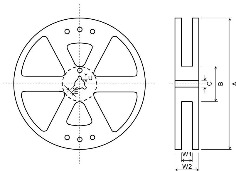
Figure 3 Reel Forms
