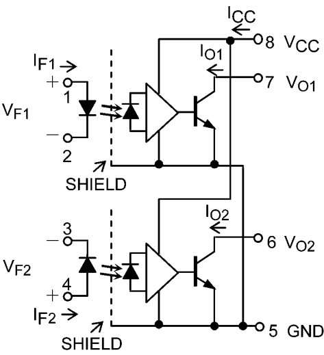
Fig. 5.1 Internal Circuit
