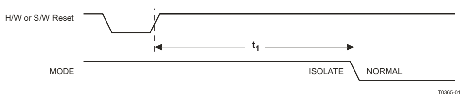
Figure 4-25. Isolation Timing
