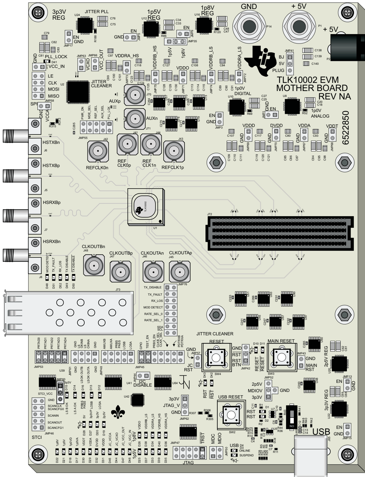
Figure 2. TLK10002EVM Motherboard
