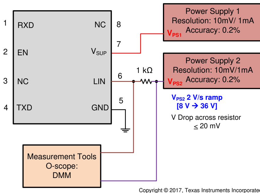
Figure 8. Test Circuit for I_{BUS\_PAS\_rec} Param 14
