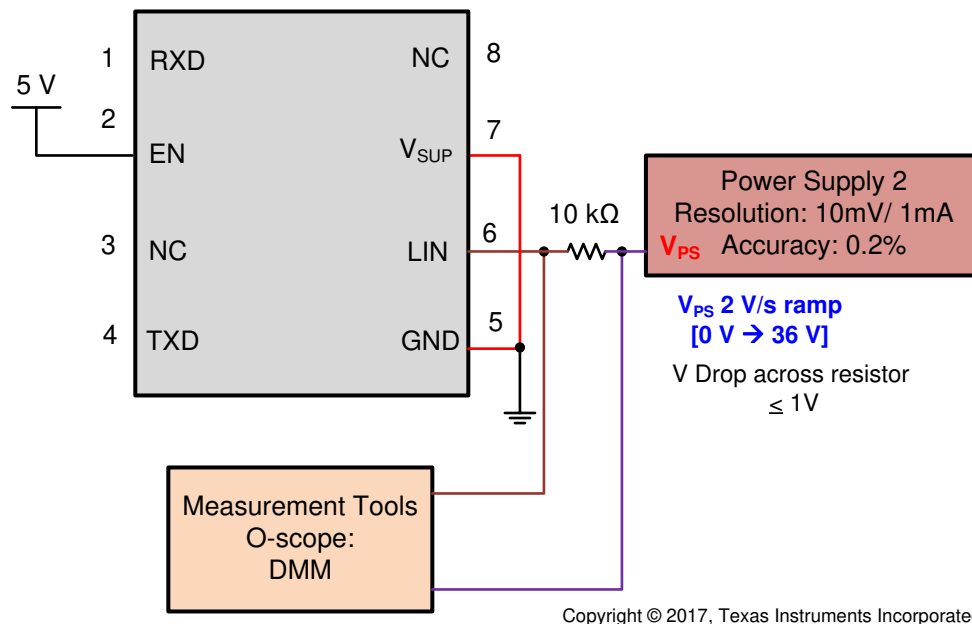
Figure 10. Test Circuit for I_{BUS\_NO\_BAT} Loss of Battery
