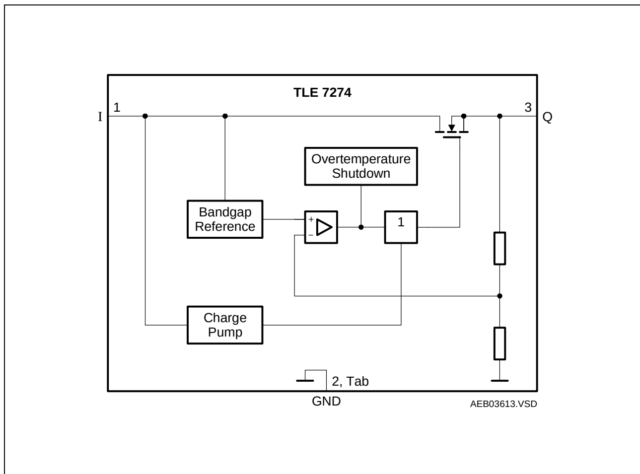
Figure 1 Block Diagram
