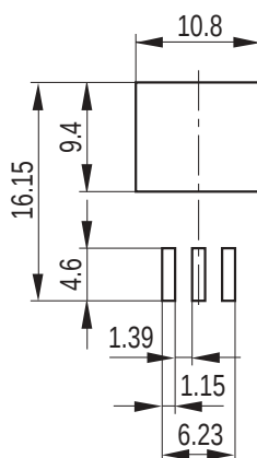
Figure 8 Foot Print for P-T0263-3-1 (Plastic Transistor Single Outline)
