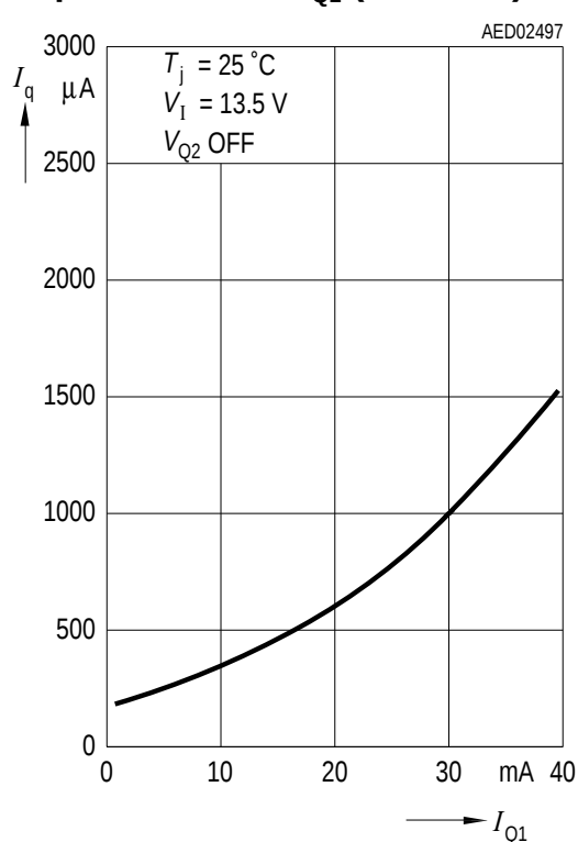
Current Consumption I_q versus Output 1 Current I_{Q1} (low load)
