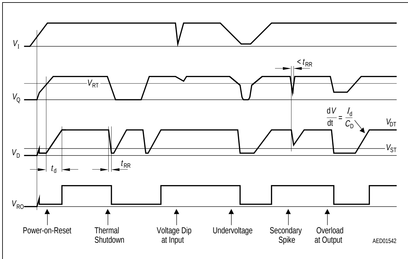
Figure 4 Reset Timing
