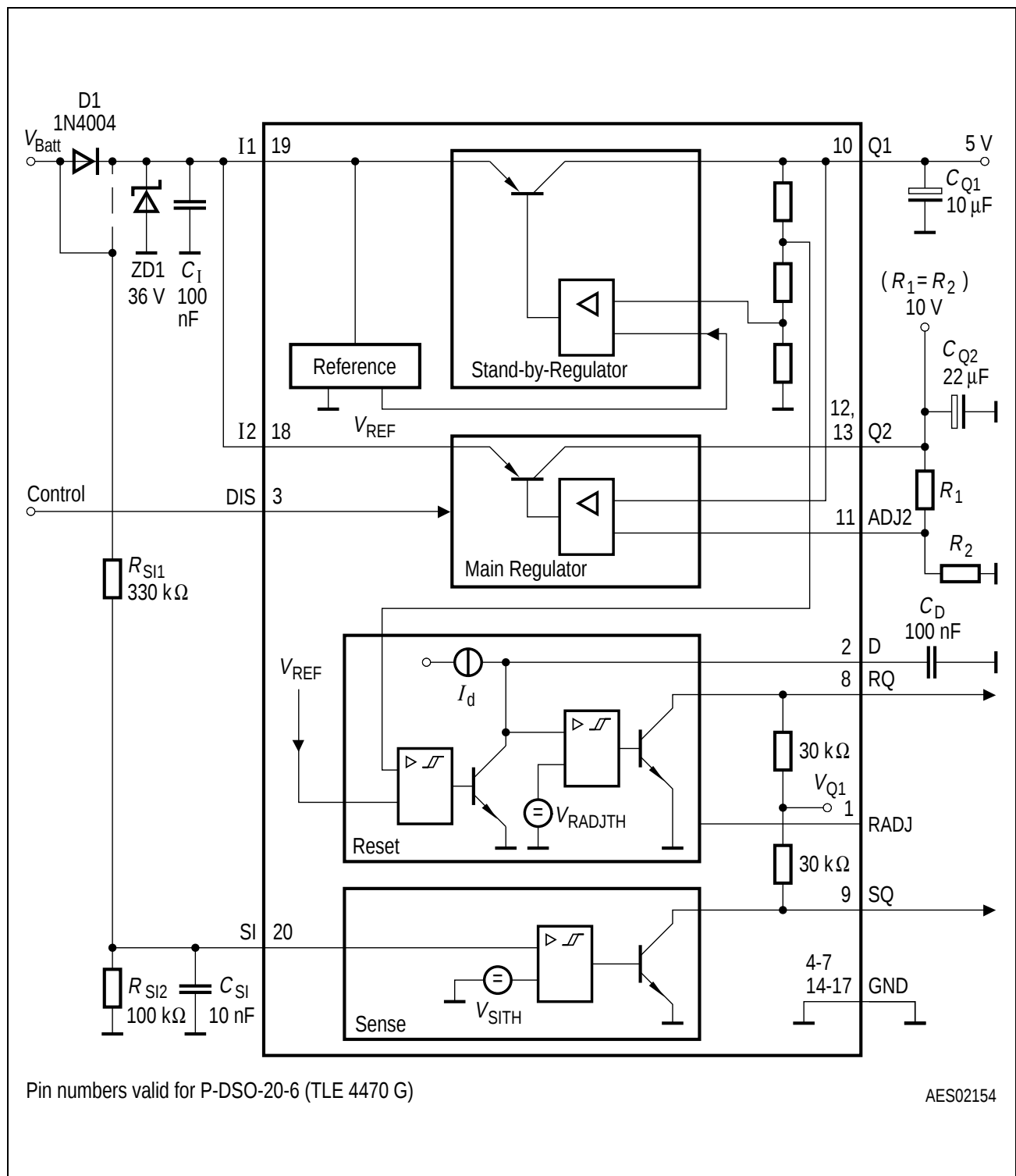
Figure 3 Application Circuit
