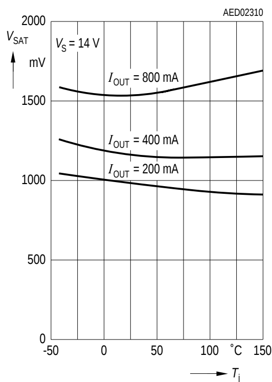
Total Drop at outputs V_{\text{SAT}} over Temperature
