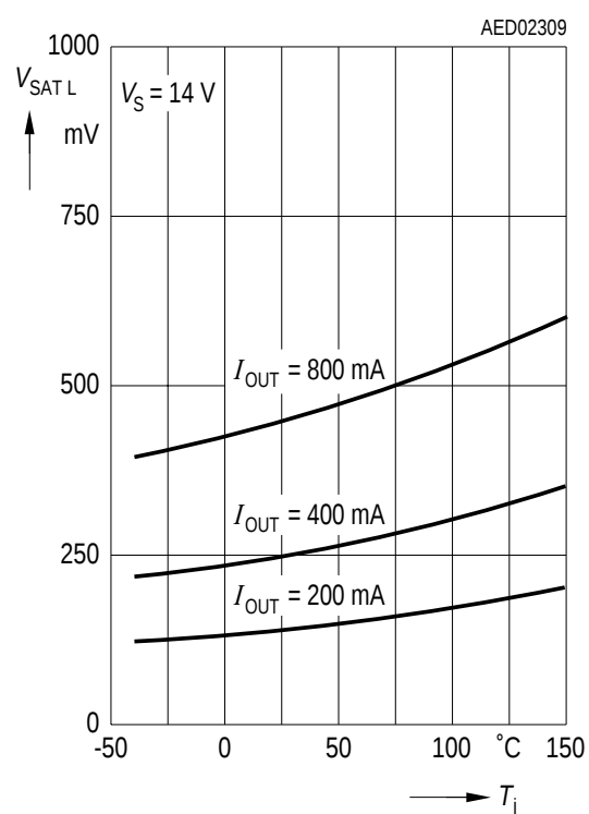
Saturation Voltage of Sink V_{\text{SAT L}} over Temperature
