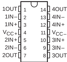
TLE2074 AND TLE2074A J OR N PACKAGE (TOP VIEW)
