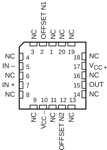
TLE2071M AND TLE2071AM FK PACKAGE (TOP VIEW)
