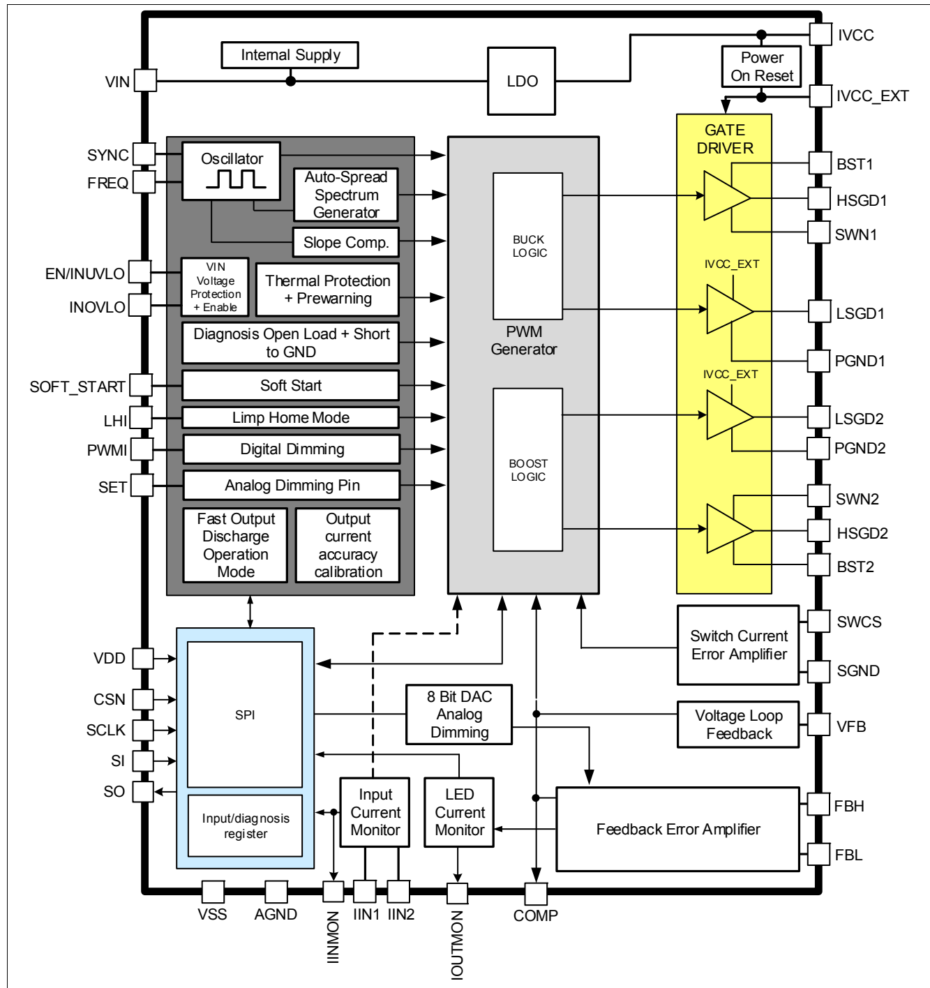
Figure 2 Block Diagram - TLD5541-1
