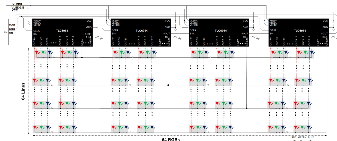
TLC6984 With Four Devices Stackable Connection
