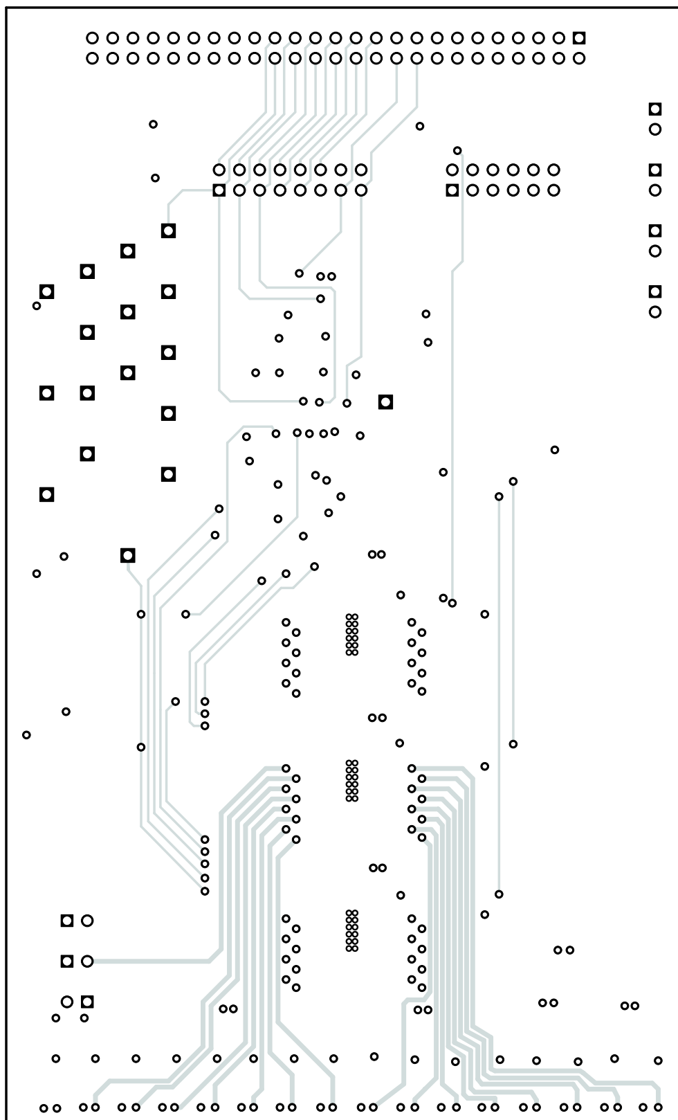
Figure 5. Layer 3 Routing
