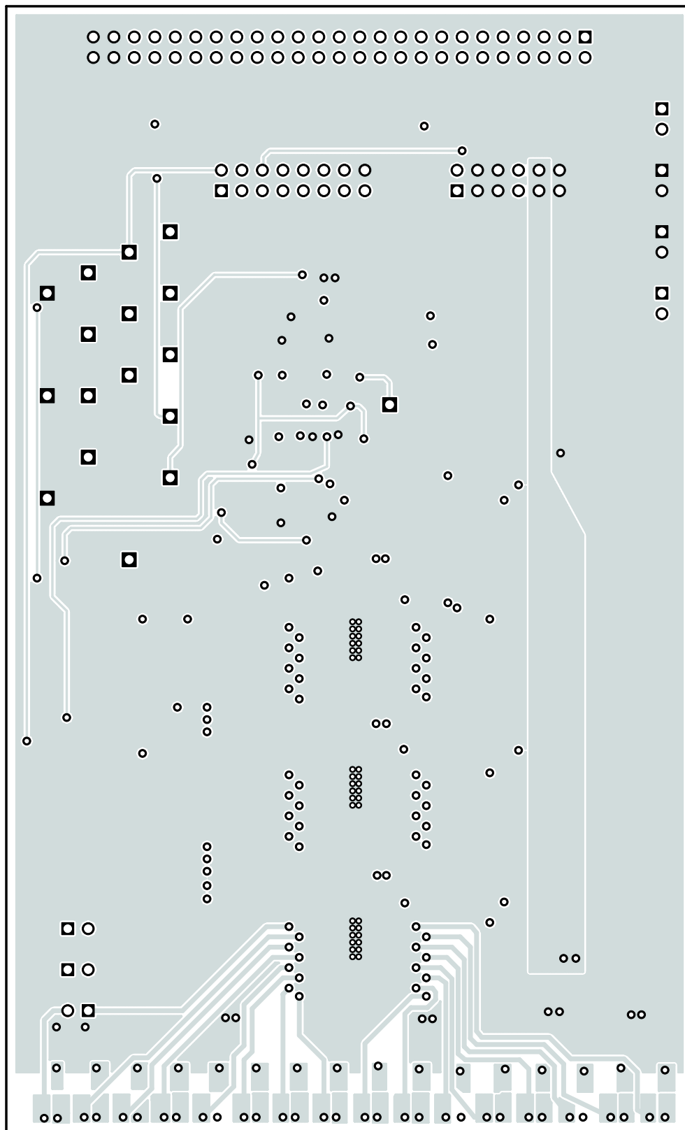
Figure 6. Bottom Layer Routing
