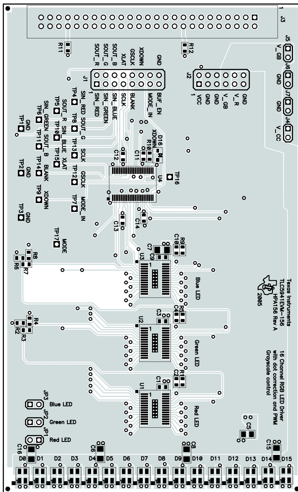
Figure 2. Assembly Layer
