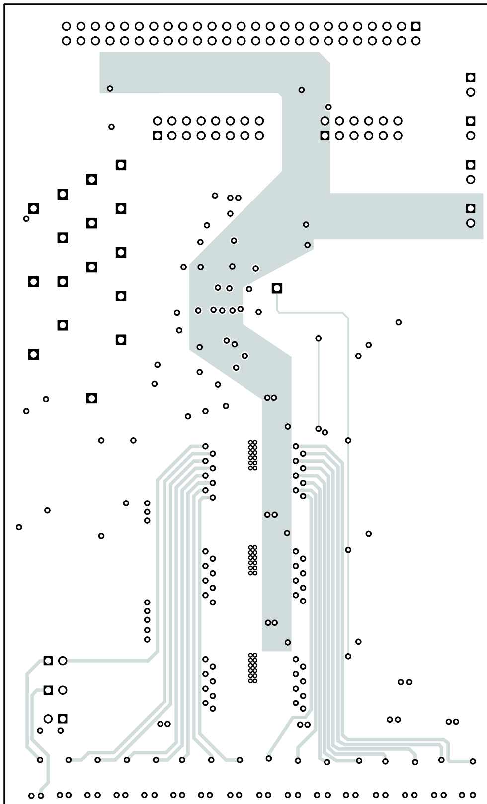
Figure 4. Layer 2 Routing
