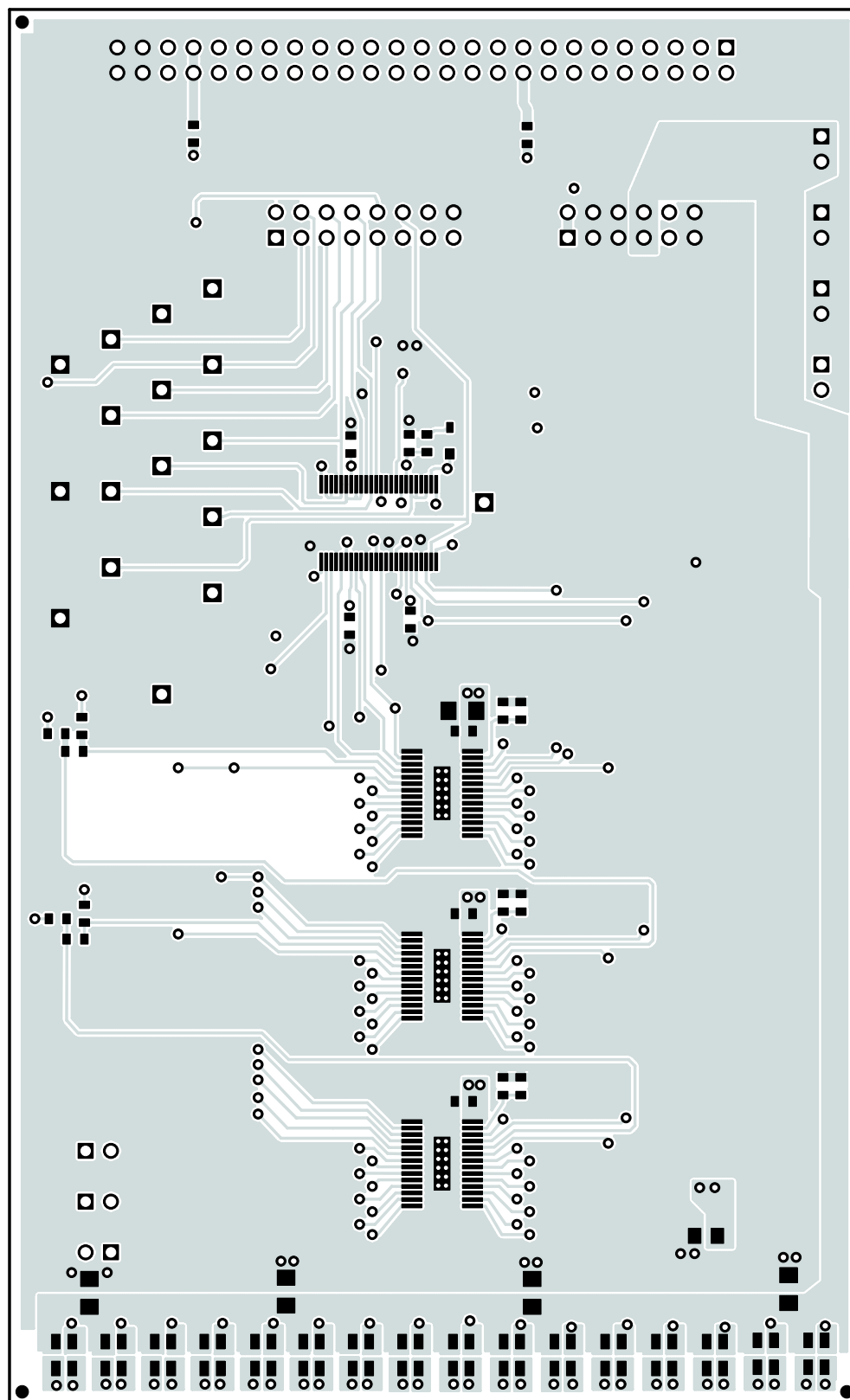
Figure 3. Top Layer Routing
