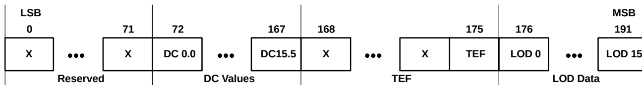
Figure 11. Status Information Data Packet Format
