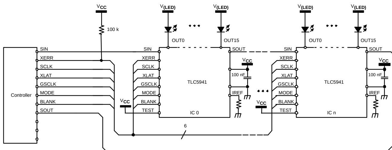
Figure 13. Cascading Devices
