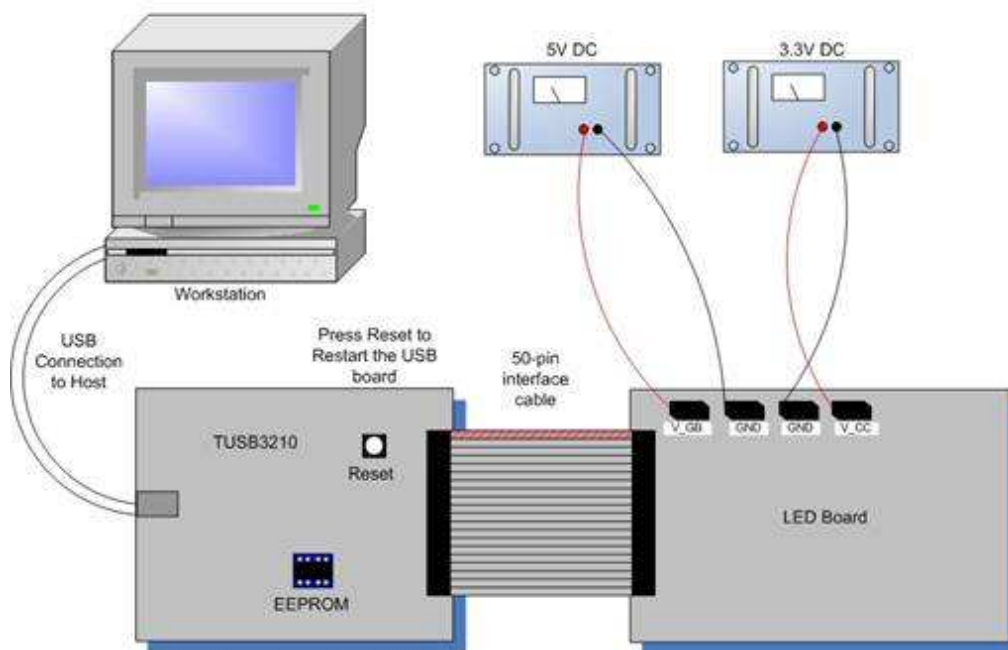
Figure 1. Hardware Setup
