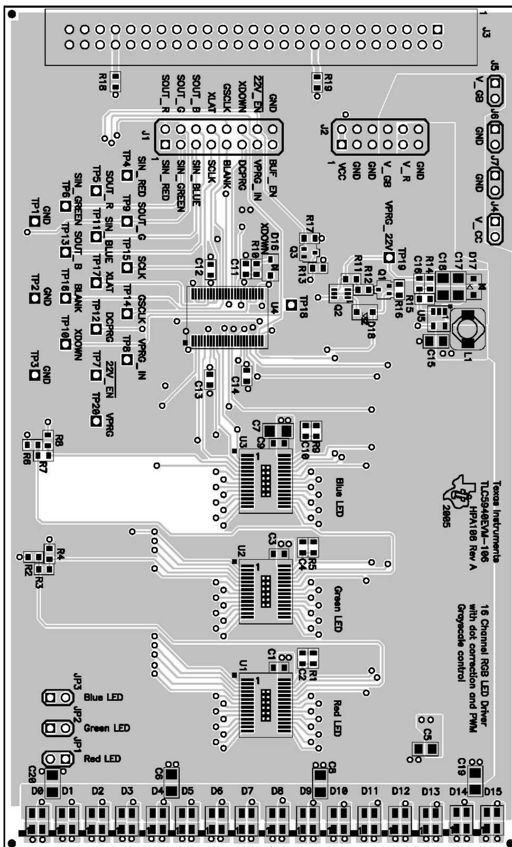
Figure 2. Assembly Layer
