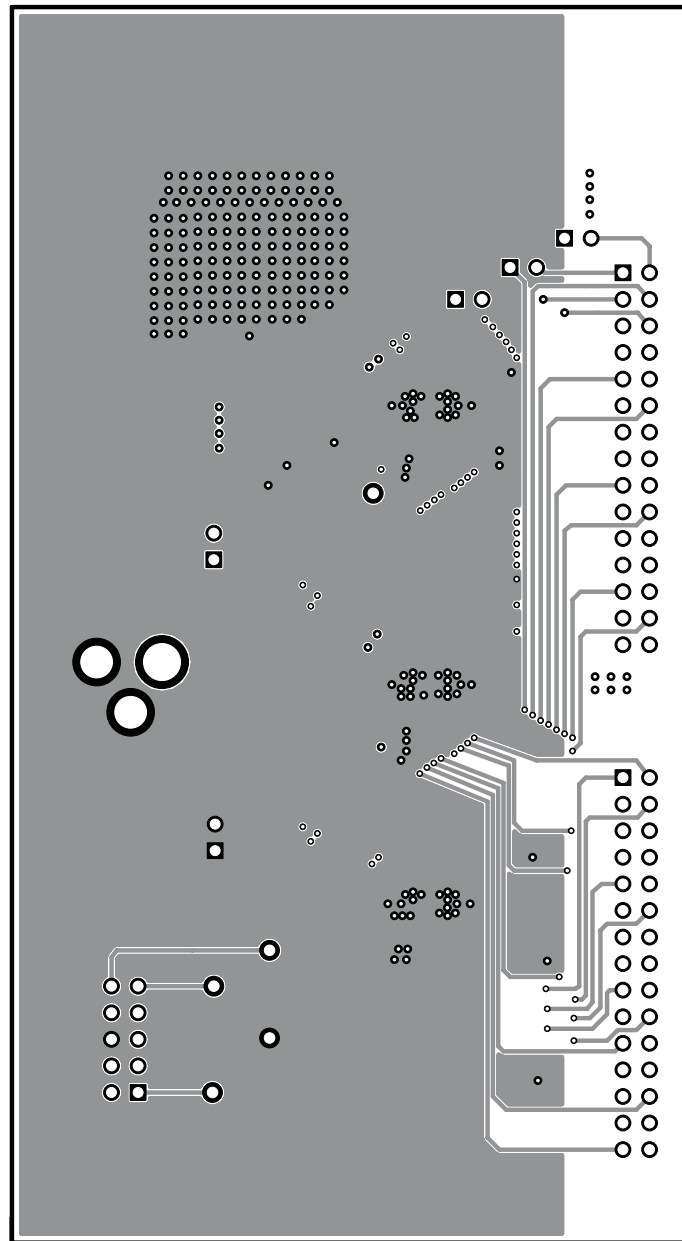
Figure 8. Layer 2 Routing
