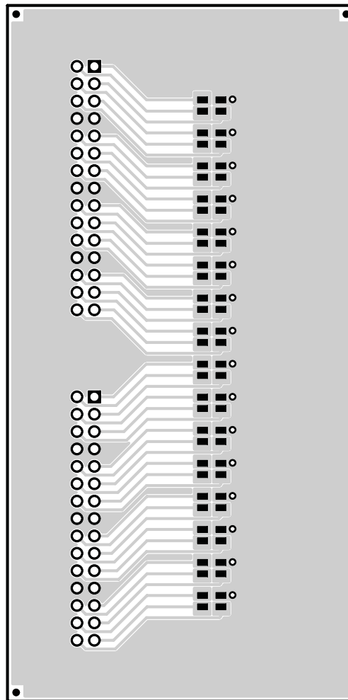
Figure 12. Top Layer Routing
