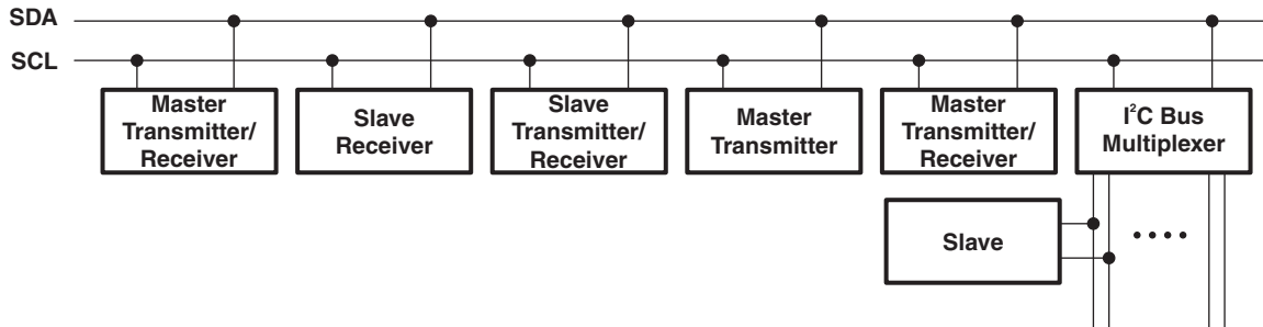
Figure 20. System Configuration
