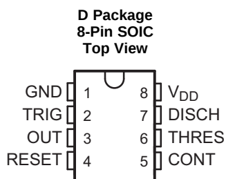
Pin Functions
