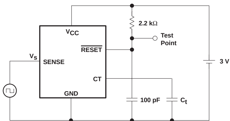
Figure 5. Switching Characteristics
