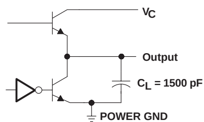
Figure 2. Switching Output Configuration and Voltage Waveform
