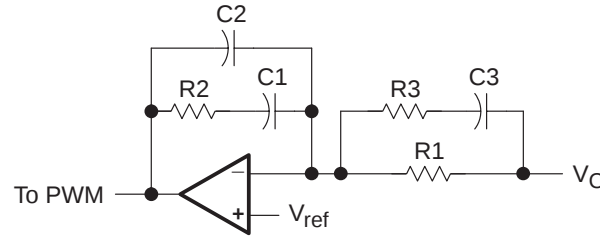
Figure 2–3. Compensation Circuit
