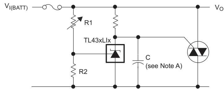
Figure 30. Crowbar Circuit
