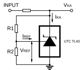
For V_{KA} \geq V_{REF}
