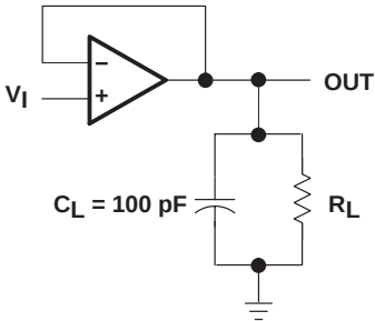
Figure 1. Unity-Gain Amplifier
