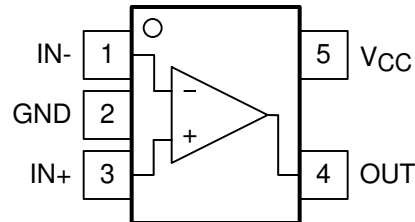
TLV331, TLV331B DBV Package 5-Pin SOT-23 Top View
