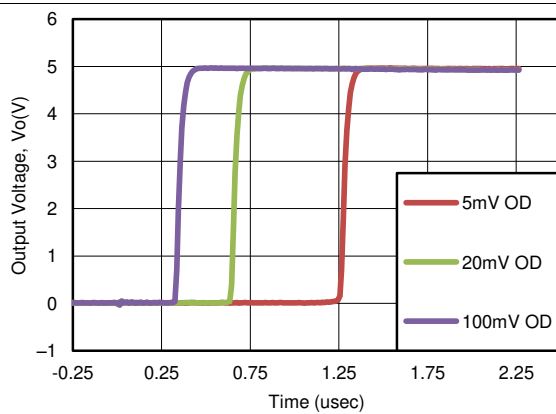
Figure 5. Response Time for Various Overdrives (Positive Transition)
