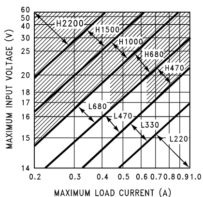
Figure 17. TL2575-12
