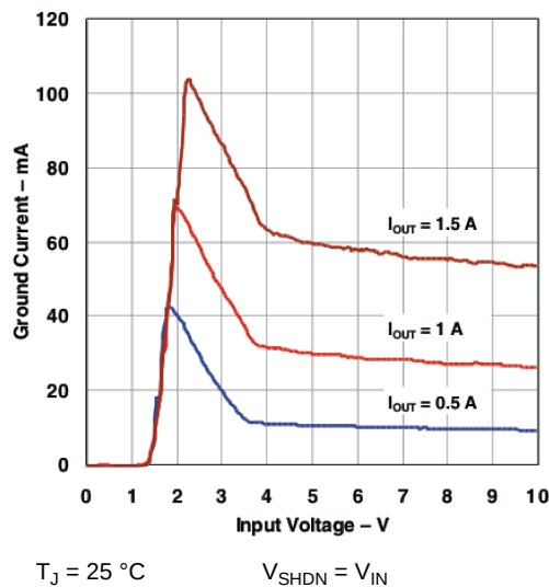
Figure 12. TL1963A-33 Ground Current vs Input Voltage
