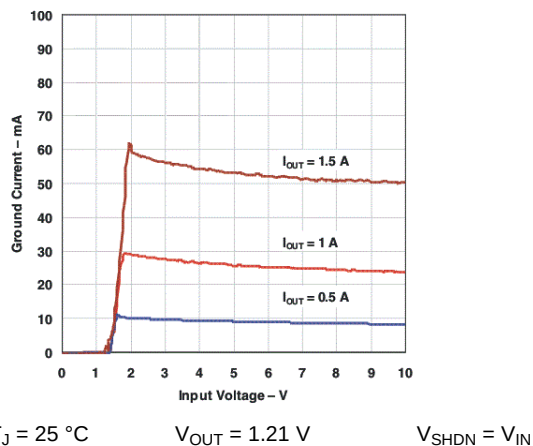
Figure 10. TL1963A Ground Current vs Input Voltage
