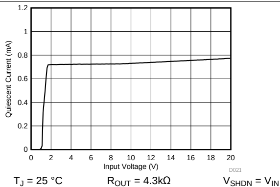
Figure 8. Quiescent Current vs Input Voltage
