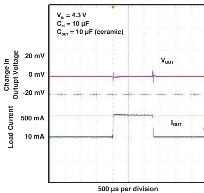
LOAD TRANSIENT RESPONSE
