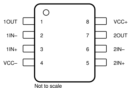
Figure 5-4. TL082x D, DDF, DGK, JG, P, PS, and PW Package 8-Pin SOIC, SOT-23 (8), VSSOP, CDIP, PDIP, SO, and TSSOP Top View
