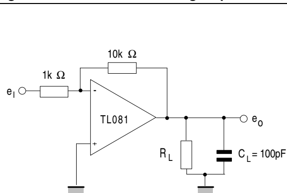
Figure 21. Gain-of-10 inverting amplifier
