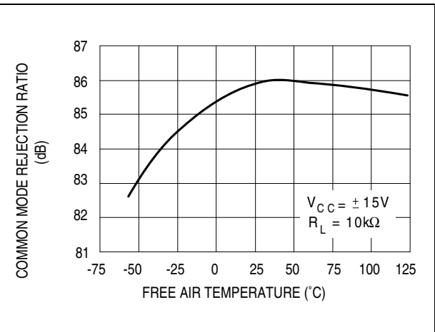
Figure 11. Common mode rejection ratio versus free air temperature
