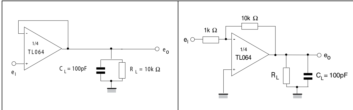
Figure 18. Gain-of-10 inverting amplifier
